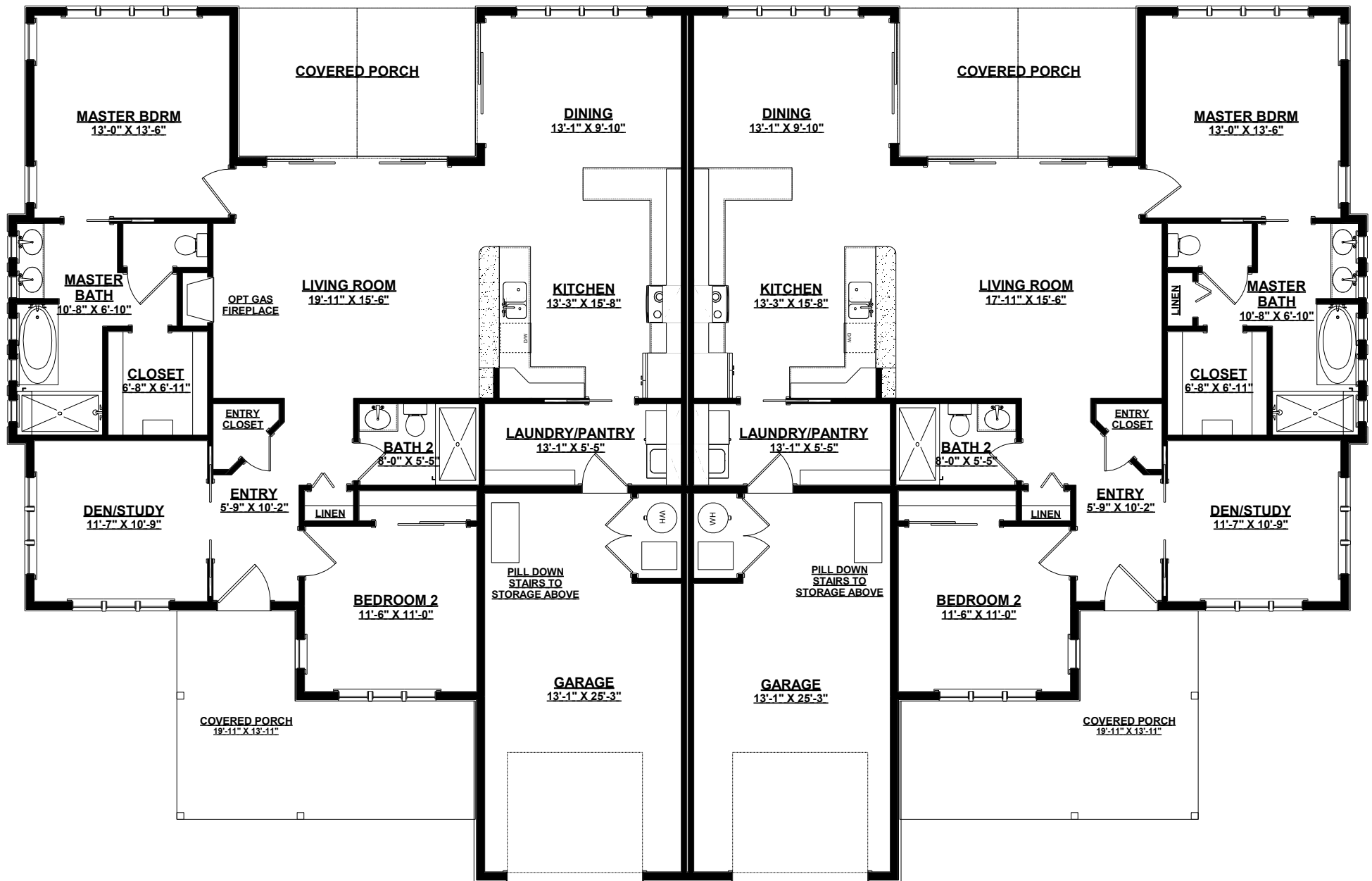
C MODEL FLOOR PLAN (1586 SQ FT X 2)
